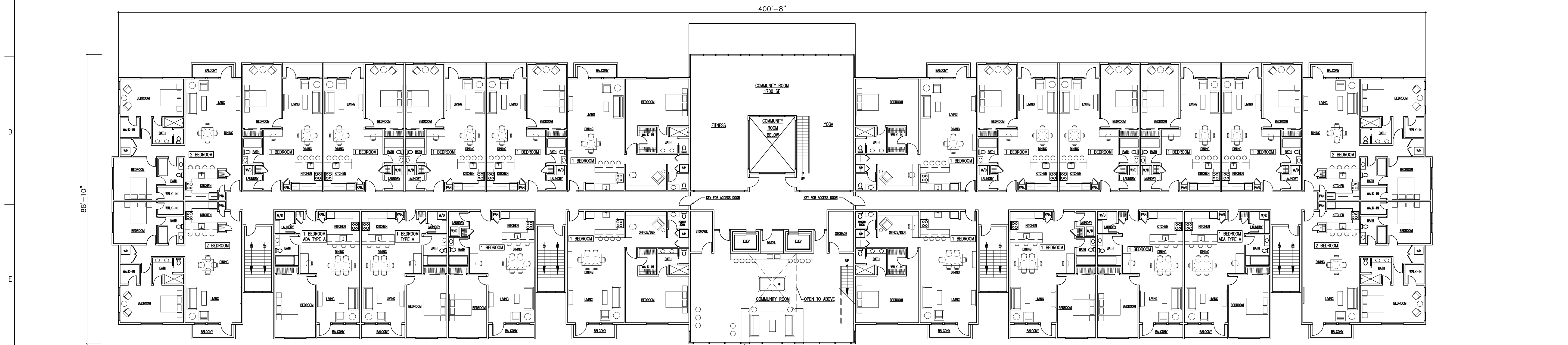
F1 PROPOSED SECOND FLOOR PLAN SCALE: 1/16" = 1'-0"
